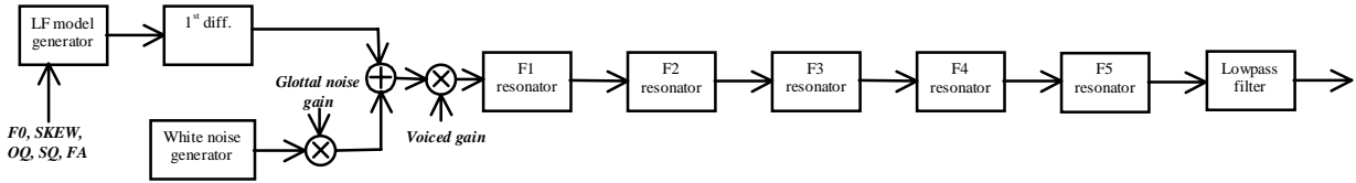
Figure 2: Formant synthesizer structure
